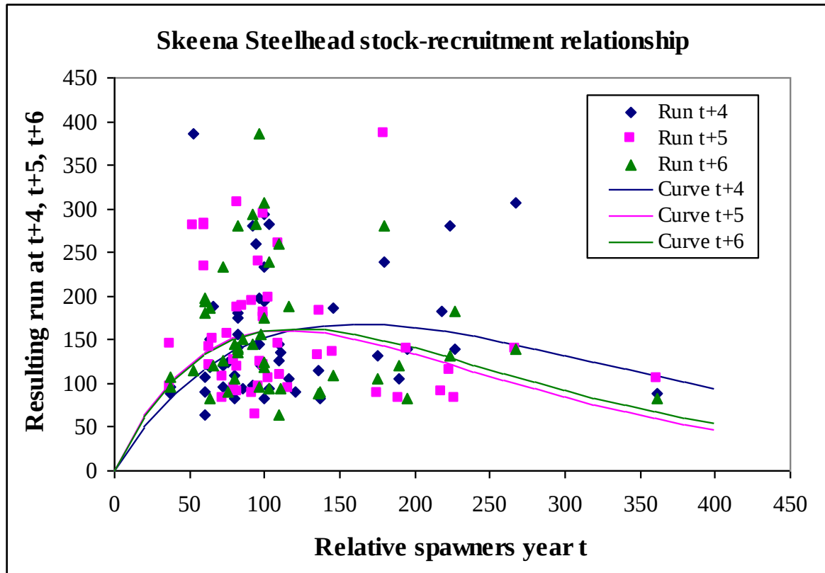
Figure 15. Stock-recruitment relationship for the overall Skeena River steelhead stock, using the Tyee test index as relative spawner abundance and calculating resulting recruits from the index inflated by estimated exploitation rates in the sockeye fishery. Three data sets and curves show that the relationship is not sensitive to whether recruits are assumed to return 4, 5, or 6 years after they were spawned. The main point of this graph is to show that the historical trend data show no indication of reduced recruitment resulting from years of low spawner abundance, i.e., no indication of recruitment overfishing for the stock complex as a whole. That would be indicated if there were data points in the lower left corner of the graph, with low numbers of spawners producing correspondingly low numbers of recruits.
